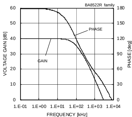
Fig. 198 Voltage Gain - Frequency ( V_{CC}/V_{EE}=+15[V]/-15[V] , A_v=40[dB] , R_L=2[k\Omega] , T_a=25[^\circ C] ) (*)The above data is ability value of sample, it is not guaranteed.
