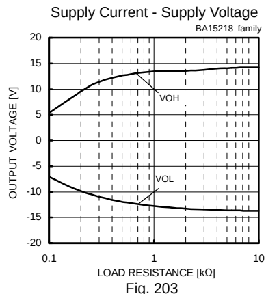
Maximum Output Voltage - Load Resistance (VCC/VEE=+15[V]/-15[V], Ta=25[°C])
