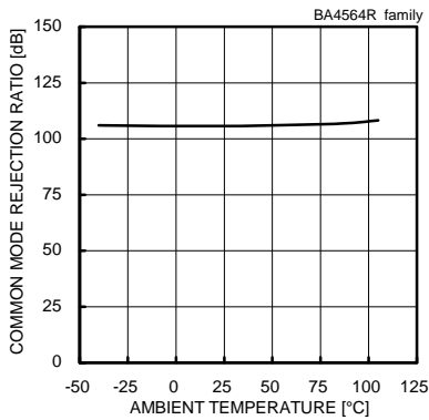
Fig. 104 Common Mode Rejection Ratio - Ambient Temperature ( V_{CC}/V_{EE}=\pm 15[V]/-15[V] , V_{icm}=-12[V] to +12[V] )
