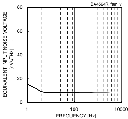
Fig. 107 Equivalent Input Noise Voltage - Frequency ( V_{CC}/V_{EE}=\pm 15[V]/-15[V] , R_s=100[\Omega] , T_a=25[^\circ C] )
