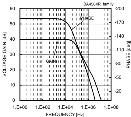
Fig. 110 Voltage Gain - Frequency ( V_{CC}/V_{EE}=\pm 15[V]/-15[V] , A_v=40[dB] , R_L=2[k\Omega] , T_a=25[^\circ C] )
