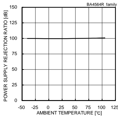
Fig. 105 Power Supply Rejection Ratio - Ambient Temperature ( V_{CC}/V_{EE}=\pm 4[V]/-4[V] to \pm 15[V]/-15[V] )
