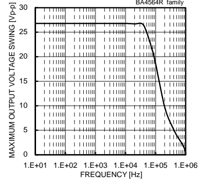
Fig. 109 Maximum Output Voltage Swing - Frequency ( V_{CC}/V_{EE}=\pm 15[V]/-15[V] , R_L=2[k\Omega] , T_a=25[^\circ C] )
