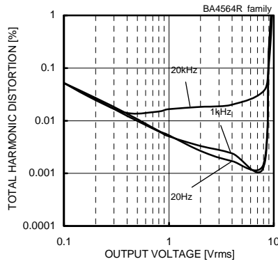
Fig. 108 Total Harmonic Distortion - Output Voltage ( V_{CC}/V_{EE}=\pm 15[V]/-15[V] , A_v=20[dB] , R_L=2[k\Omega] , 80[kHz] -LPF, T_a=25[^\circ C] )
