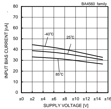
Fig. 55 Input Bias Current - Supply Voltage (Vicm=0[V], Vout=0[V])
