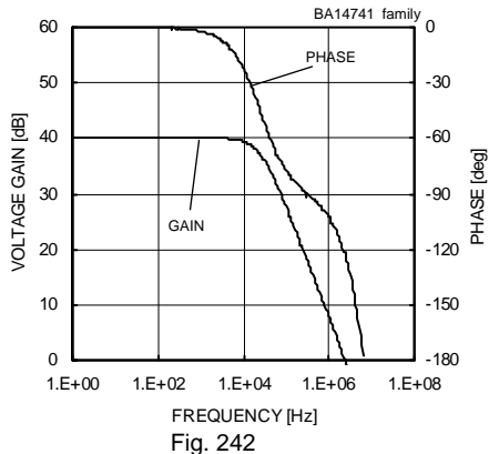
Fig. 242 Voltage Gain - Frequency ( V_{CC}/V_{EE}=+15[V]/-15[V] , A_v=40[dB] , R_L=2[kΩ] , T_a=25[°C] )
