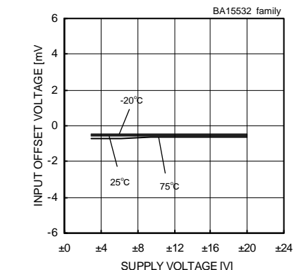
Fig. 251 Input Offset Voltage - Supply Voltage (Vicm=0[V], Vout=0[V])
