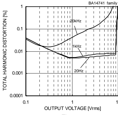
Fig. 240 Total Harmonic Distortion - Output Voltage ( V_{CC}/V_{EE}=+15[V]/-15[V] , A_v=20[dB] , R_L=2[kΩ] , 80[kHz] -LPF, T_a=25[°C] )
