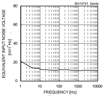
Fig. 239 Equivalent Input Noise Voltage - Frequency ( V_{CC}/V_{EE}=+15[V]/-15[V] , R_s=100[Ω] , T_a=25[°C] )
