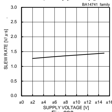
Fig. 238 Slew Rate - Supply Voltage ( C_L=100[pF] , R_L=2[kΩ] , T_a=25[°C] )
