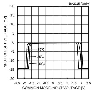
Fig. 302 Input Offset Voltage - Common Mode Input Voltage ( V_{CC}/V_{EE}=+2.5[V]/-2.5[V] , V_{out}=0[V] )
