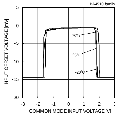
Fig. 279 Input Offset Voltage - Common Mode Input Voltage ( V_{CC}/V_{EE}=2.5[V]/-2.5[V] )
