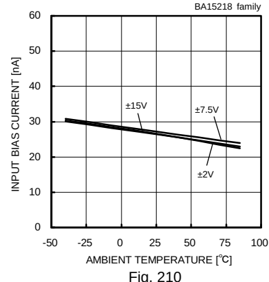
Input Bias Current - Ambient Temperature (V icm =0[V], V out =0[V])
