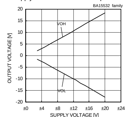
Maximum Output Voltage - Supply Voltage (RL=600[Ω], Ta=25[°C])
