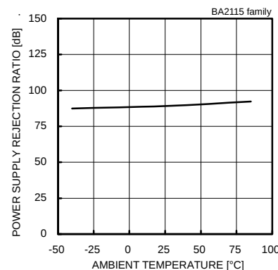
Fig. 305 Power Supply Rejection Ratio - Ambient Temperature ( V_{CC}/V_{EE}=+2.5[V]/-2.5[V] )
