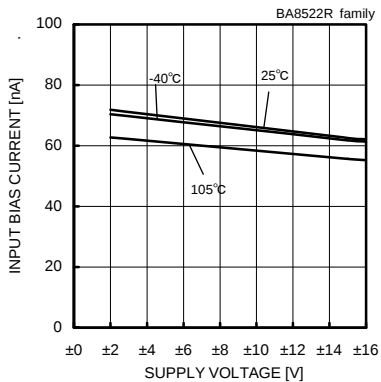
Fig. 187 Input Bias Current - Supply Voltage (Vicm=0V, Vout=0V)
