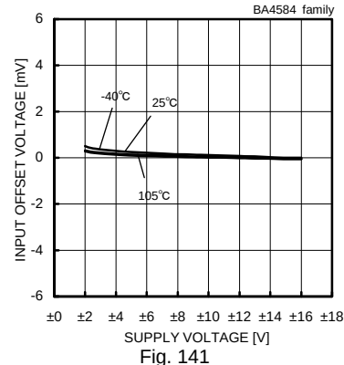
Fig. 141 Input Offset Voltage - Supply Voltage (Vicm=0[V], Vout=0[V])
