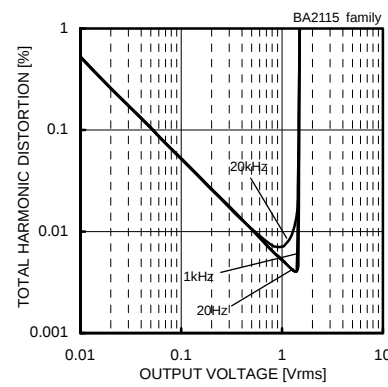
Fig. 308 Total Harmonic Distortion - Output Voltage ( V_{CC}/V_{EE}=2.5[V]/-2.5[V] , R_L=3[k\Omega] , 80[kHz]-LPF, T_a=25[^\circ C] )
