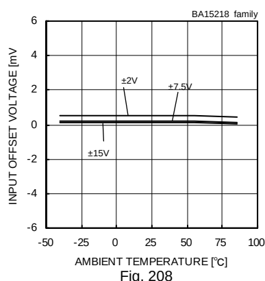
Input Offset Voltage - Ambient Temperature (V icm =0[V], V out =0[V])
