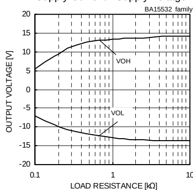
Maximum Output Voltage - Load Resistance (VCC/VEE=+15[V]/-15[V], Ta=25[°C])
