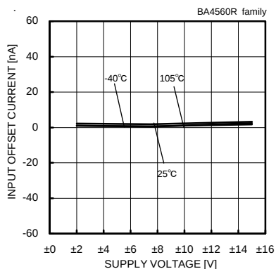
Fig. 79 Input Offset Current - Supply Voltage ( V_{icm}=0[V] , V_{out}=0[V] )
