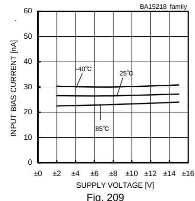
Input Bias Current - Supply Voltage (V icm =0[V], V out =0[V])
