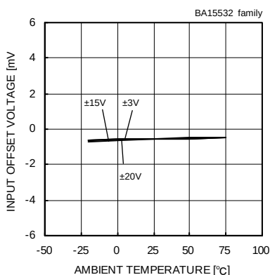
Input Offset Voltage - Ambient Temperature (Vcm=0[V], Vout=0[V])
