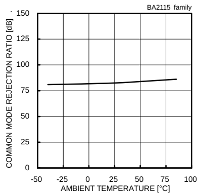
Fig. 304 Common Mode Rejection Ratio - Ambient Temperature ( V_{CC}/V_{EE}=+2.5[V]/-2.5[V] )
