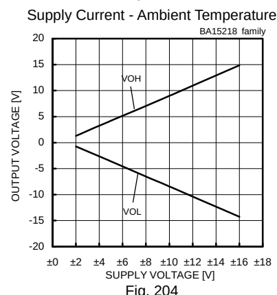
Maximum Output Voltage - Supply Voltage (R L =2[kΩ], T a =25[°C])
