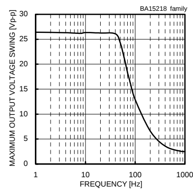
Fig. 219 Maximum Output Voltage Swing - Frequency ( V_{CC}/V_{EE}=+15[V]/-15[V] , R_L=2[k\Omega] , T_a=25[^\circ C] )
