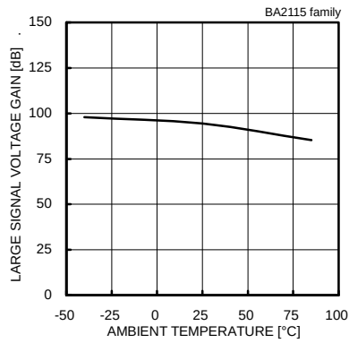
Fig. 303 Large Signal Voltage Gain - Ambient Temperature ( V_{CC}/V_{EE}=+2.5[V]/-2.5[V] )
