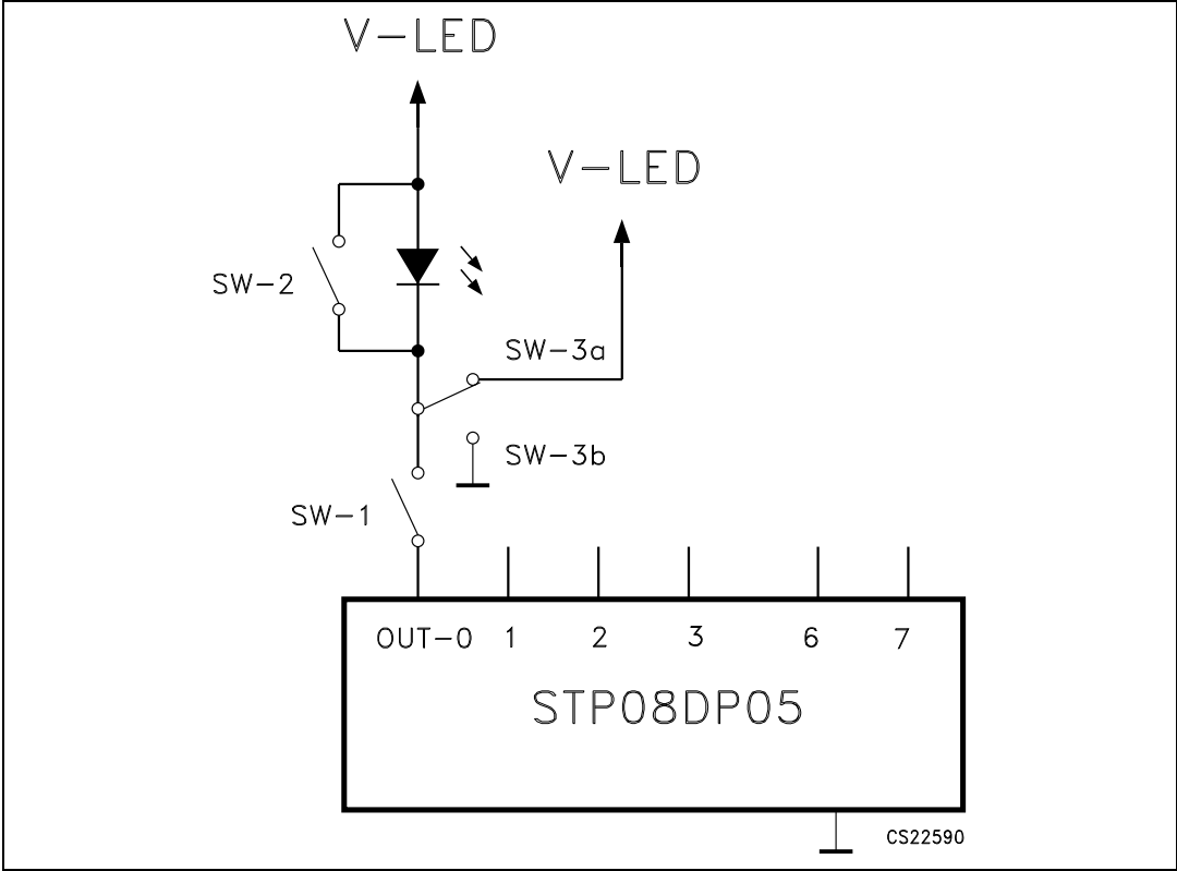
Figure 20. Detection circuit
