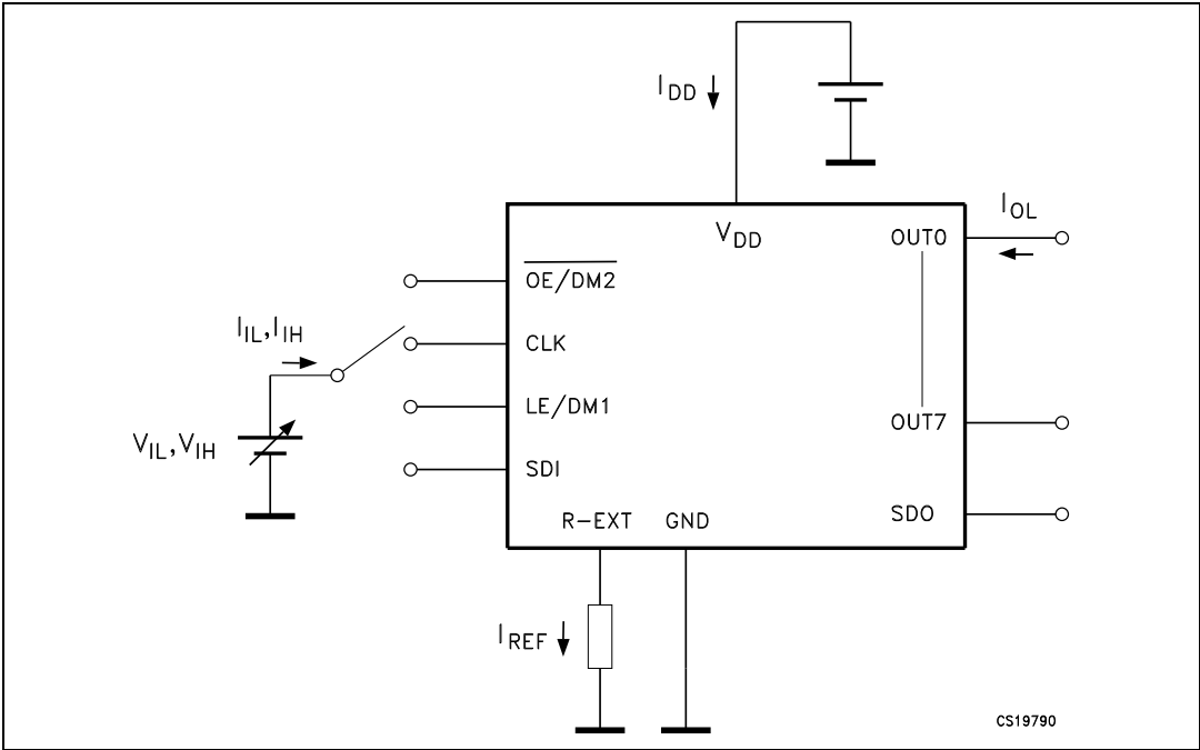
Figure 14. DC characteristics
