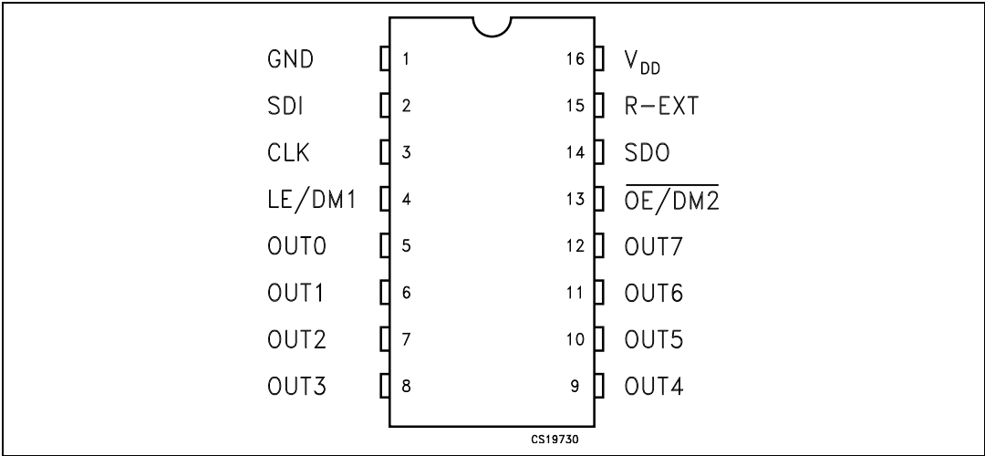
Figure 1. Connections diagram
