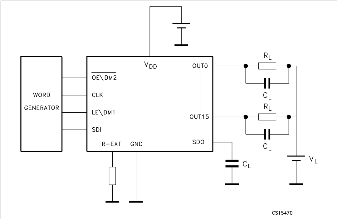
Figure 15. AC characteristics
