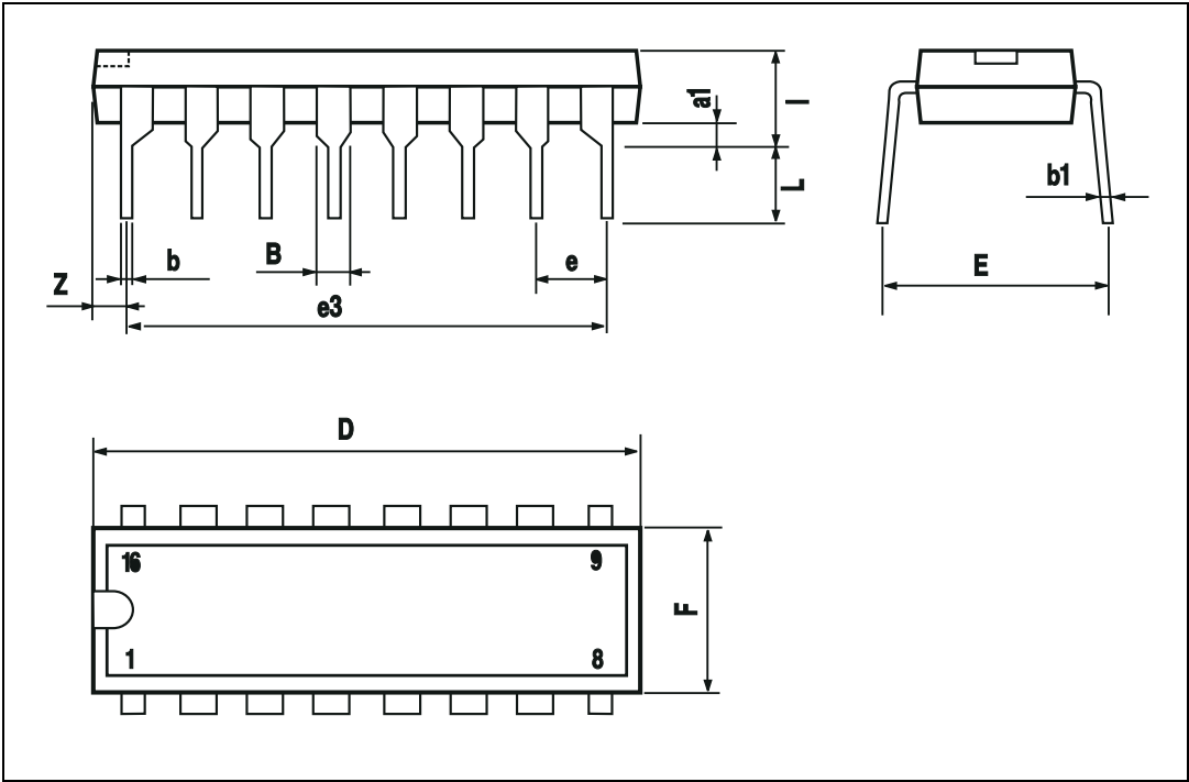
Figure 21. DIP16 drawing
