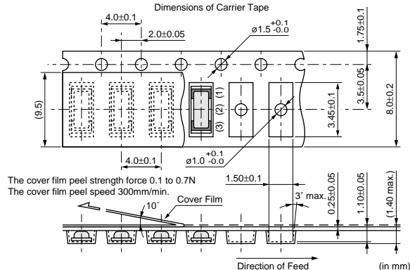
CSTCE_V(A)
