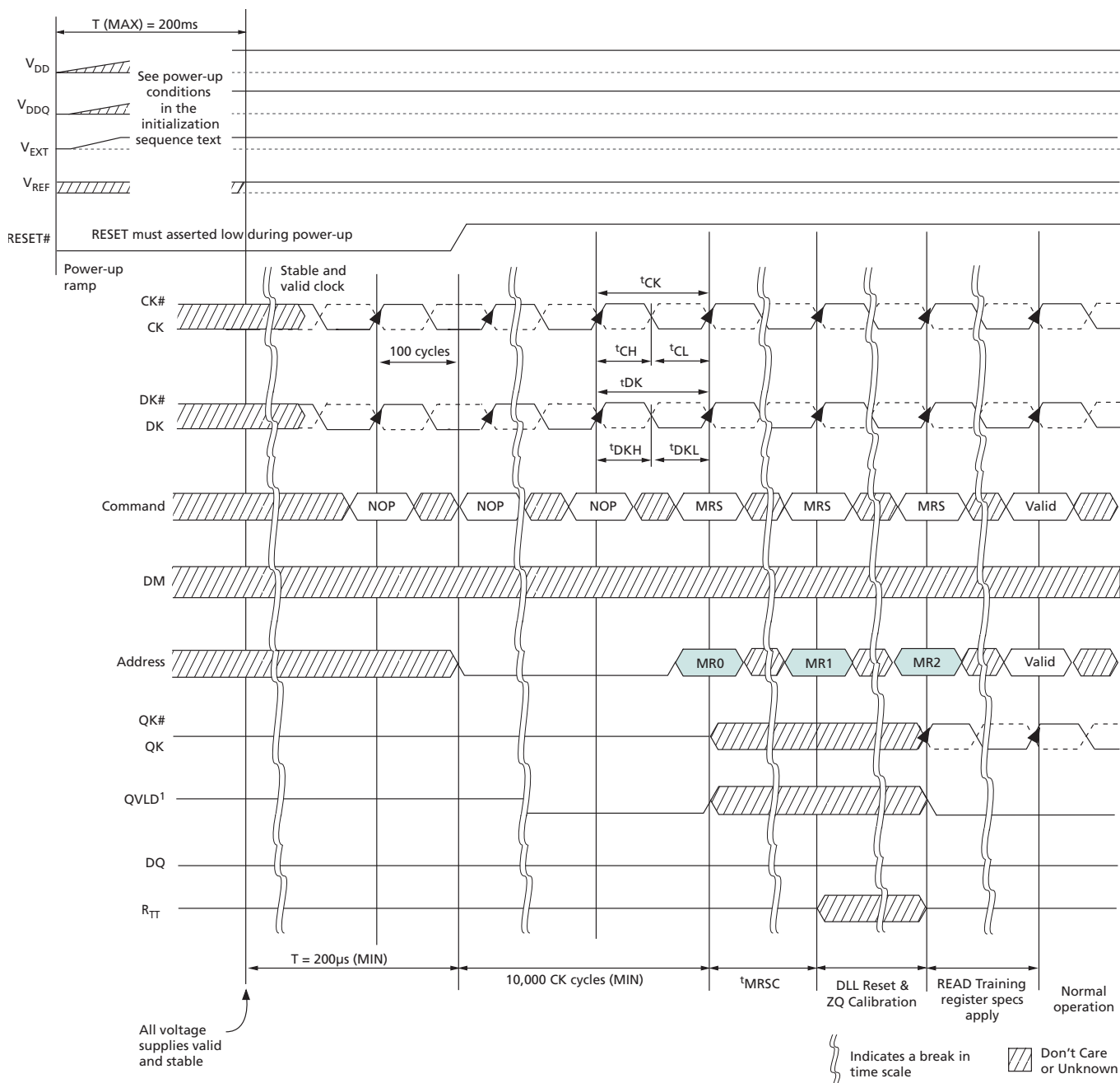
Figure 42: Power-Up/Initialization Sequence
