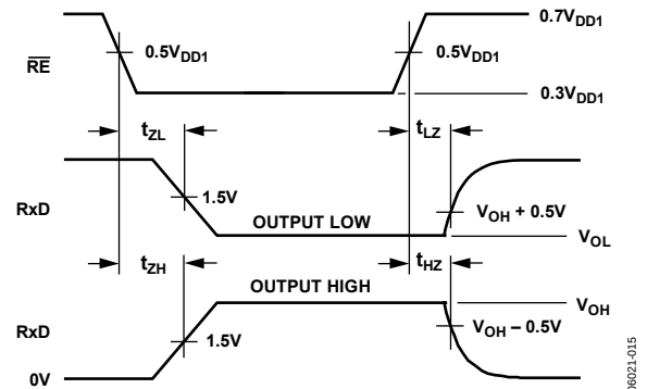
Figure 5. Receiver Enable/Disable Timing
