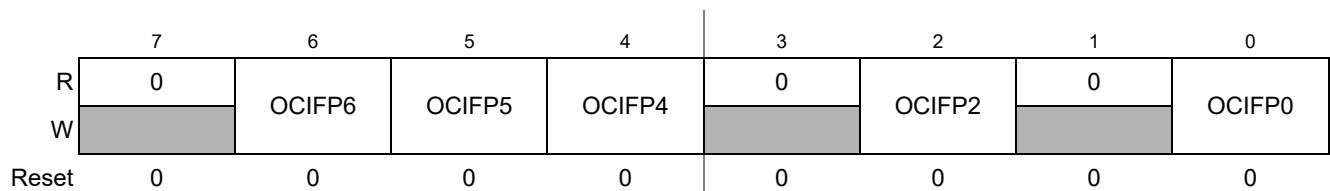
Figure 2-23. Port P Over-Current Interrupt Flag Register
