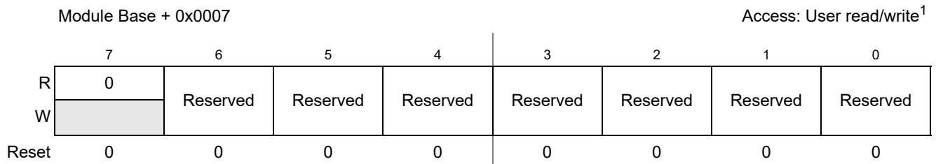
Figure 19-5. Reserved Registerfv_dac_8b5v_RESERVED
