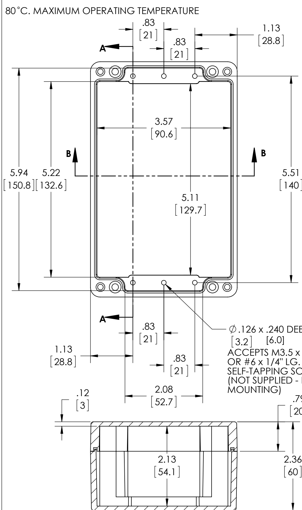
SECTION B-B
