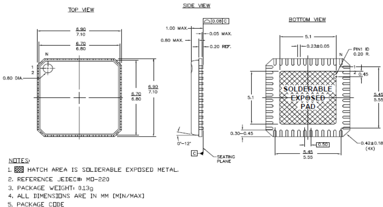
Figure 15. 48-Pin (7 × 7 × 1.0 mm) QFN
