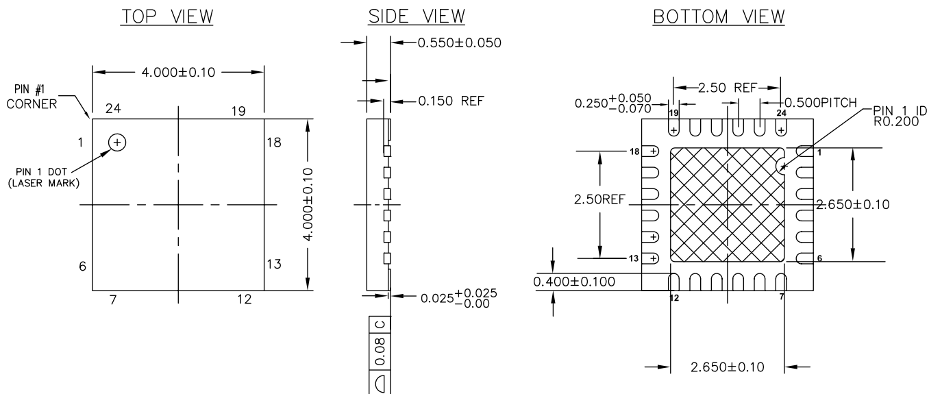
Figure 17. 24-Pin (4 × 4 × 0.55 mm) Sawn QFN
