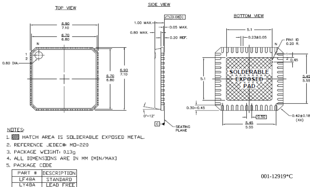
Figure 15. 48-Pin (7 × 7 × 1.0 mm) QFN
