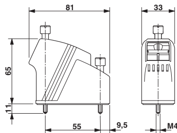
Dimensioned drawing
