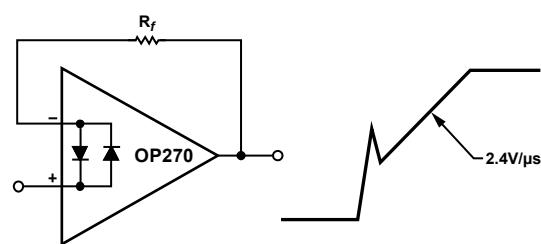
Figure 40. Pulsed Operation
