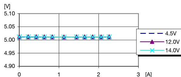
Output voltage vs. load current at T_{ref} = +25^{\circ}\text{C}
