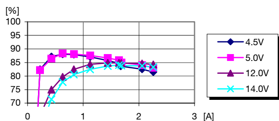
Efficiency vs. load current and input voltage at T_{ref} = +25^{\circ}\text{C}
