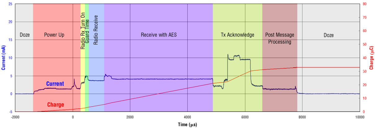
Atomic Operation—Maximum Length Receive with Acknowledge, 7.25ms Time Slot (32.6µC Total Charge at 3.6V)
