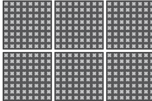
Tiled Matrices
