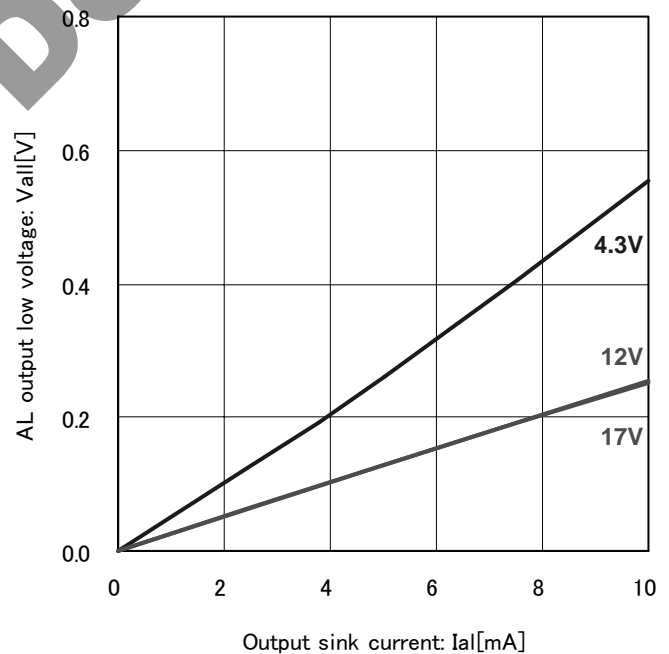
Fig.14 AL output low voltage ( T_a=25^{\circ}\text{C} )
