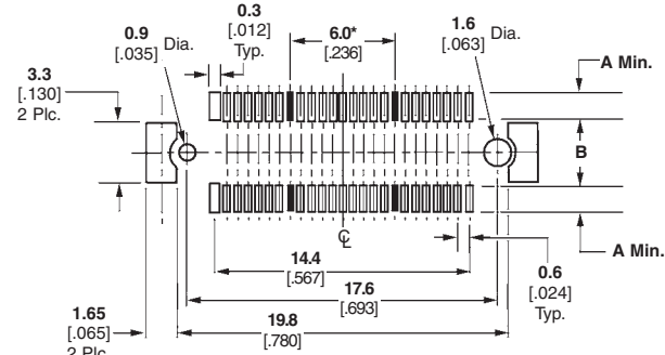
For 50-Position Receptacles *Spacing between grounding circuits
