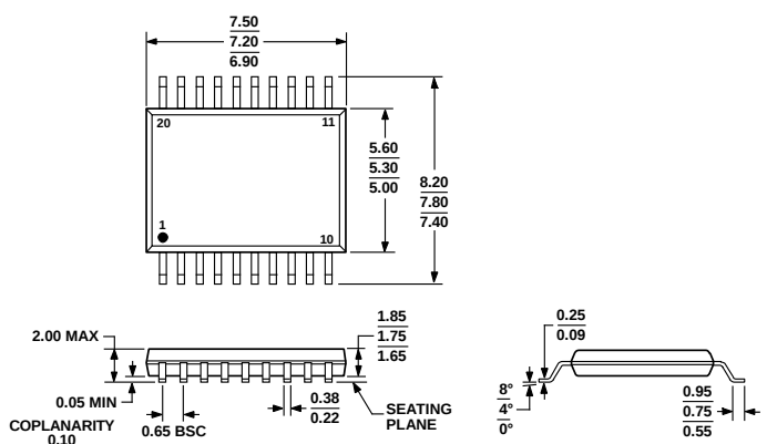
COMPLIANT TO JEDEC STANDARDS MO-150-AE Figure 18. 20-Lead Shrink Small Outline Package [SSOP] (RS-20) Dimensions shown in millimeters
