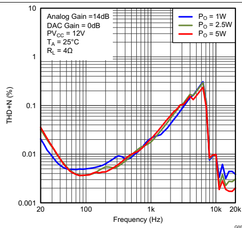
Figure 3. Total Harmonic Distortion + Noise vs Frequency
