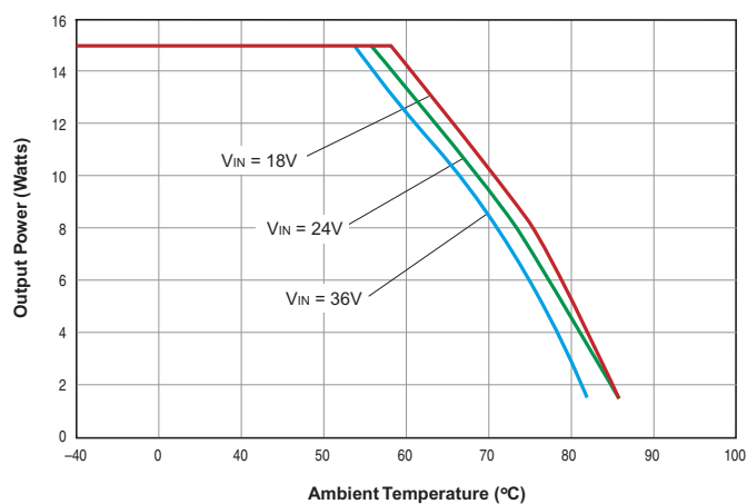
BWR-5/1500-D24A Output Power vs. Ambient Temperature (No air flow)
