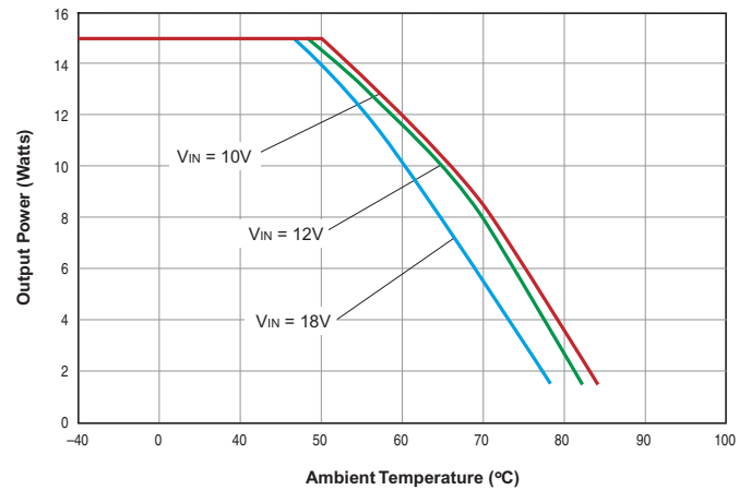
BWR-5/1500-D12A Output Power vs. Ambient Temperature (No air flow)
