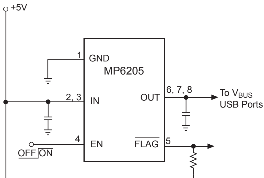
Figure 3—Application Circuit
