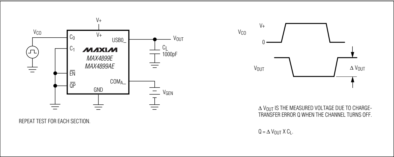
Figure 5. Charge Injection
