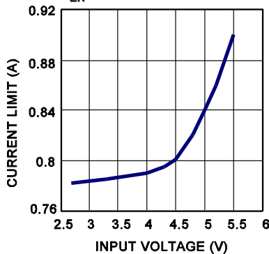
Current Limit vs. Input Voltage V_{EN}=5V
