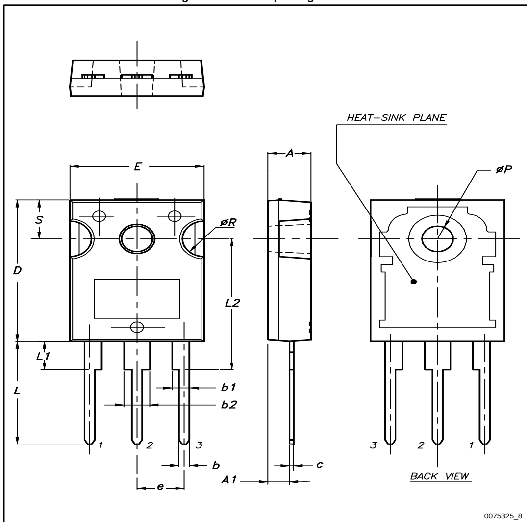
Figure 15: TO-247 package outline
