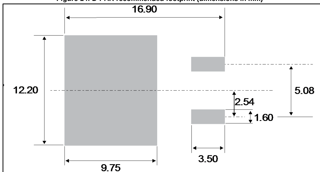
Figure 14: D 2 PAK recommended footprint (dimensions in mm)
