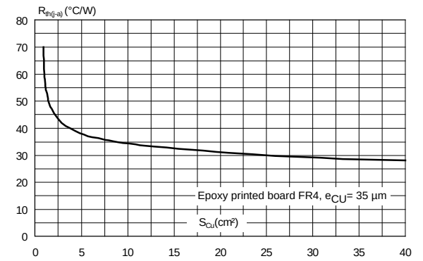
Figure 12: Thermal resistance, junction to ambient, versus copper surface under tab (D²PAK)
