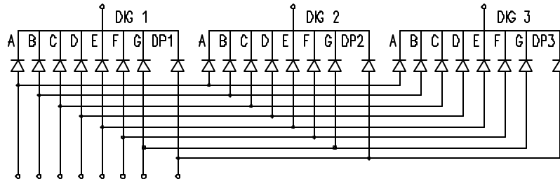
COMMON CATHODE
