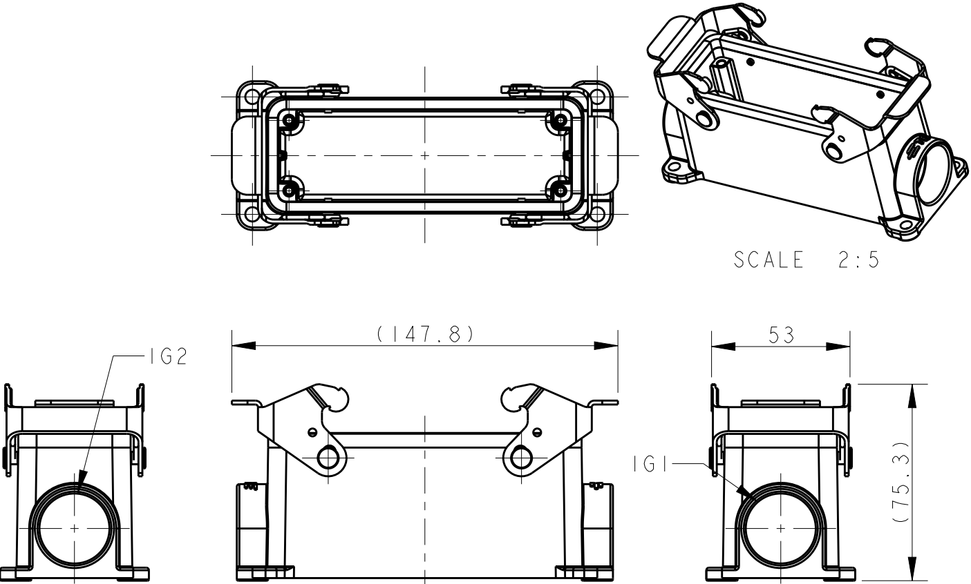
TYPE 3: BODY + STEEL LOCKING SIDE ENTRY OTHER SPEC REFER TO TYPE 1
