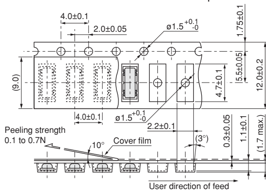
Dimensions of Carrier Tape
