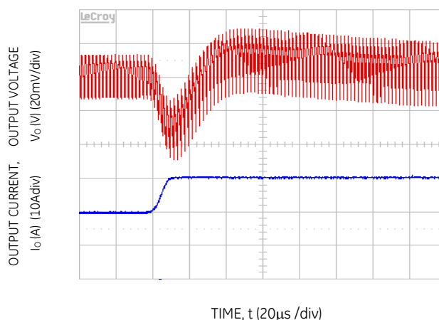
Figure 16. Transient Response to Dynamic Load Change from 50% to 100% at 12Vin, C_{out}= 2\times 47\mu\text{F} + 3\times 330\mu\text{F} , C_{Tune}=5600\text{pF} & R_{Tune}=220\text{ ohms}
