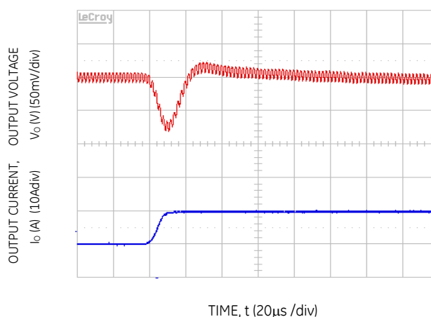
Figure 34. Transient Response to Dynamic Load Change from 50% to 100% at 12Vin, C_{out}=8 \times 47 \mu\text{F} , C_{Tune}=1500\text{pF} & R_{Tune}=220 \text{ ohms}
