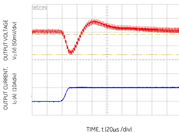
Figure 28 Transient Response to Dynamic Load Change from 50% to 100% at 12Vin, C_{out}= 5 \times 47\mu\text{F} + 1 \times 330\mu\text{F} , C_{Tune}=2200\text{pF} & R_{Tune}=220\text{ ohms}
