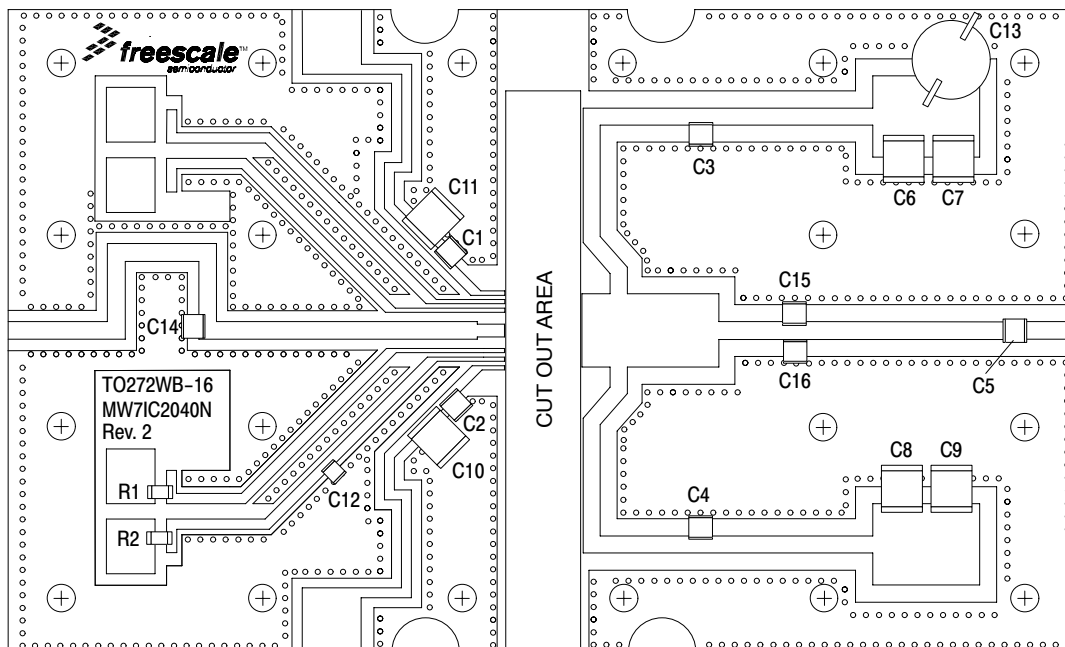
Figure 21. MW71C2040NR1(GNR1)(NBR1) Test Circuit Component Layout — 1805-1880 MHz
