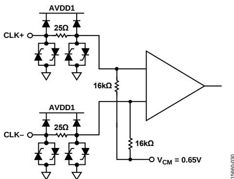
Figure 58. Clock Inputs
