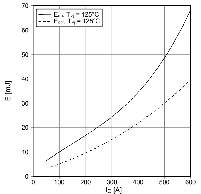
Schaltverluste IGBT-Wechselr. (typisch) switching losses IGBT-inverter (typical) E_{on} = f(I_C), E_{off} = f(I_C) V_{GE} = \pm 15\text{ V}, R_{Gon} = 2.7\ \Omega, R_{Goff} = 2.7\ \Omega, V_{CE} = 600\text{ V}
