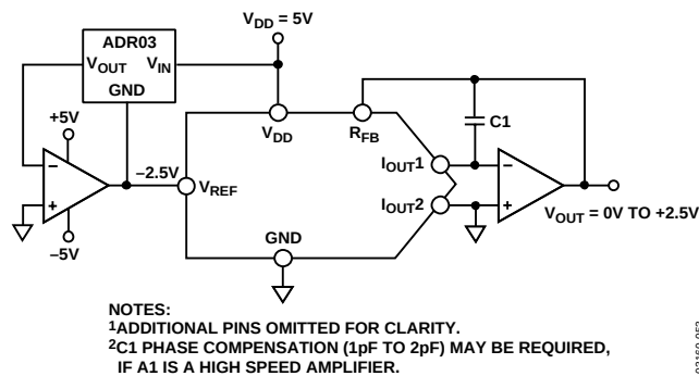
Figure 53. Positive Voltage Output with Minimum of Components
