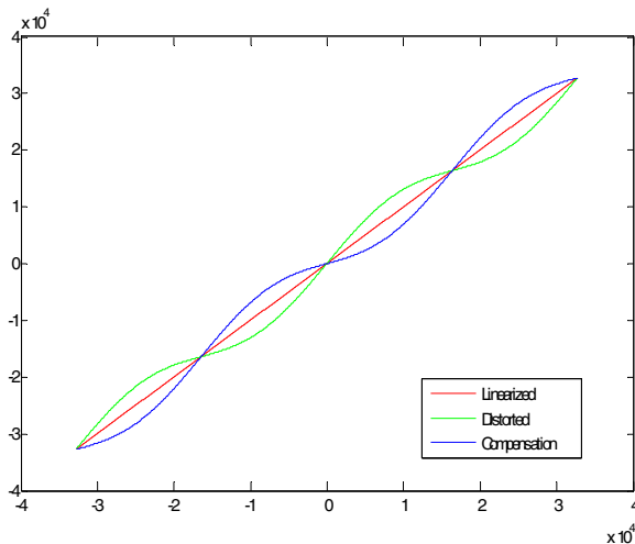
Fig. 3–4: Linearization - Principle
