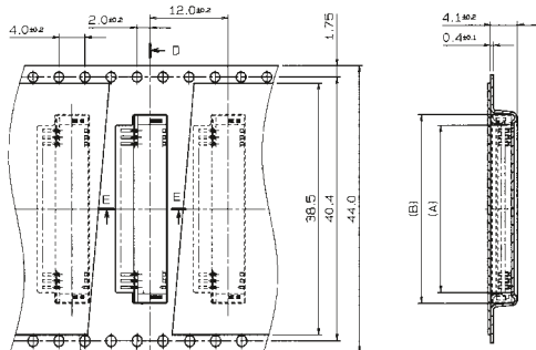
SECT. D-D
