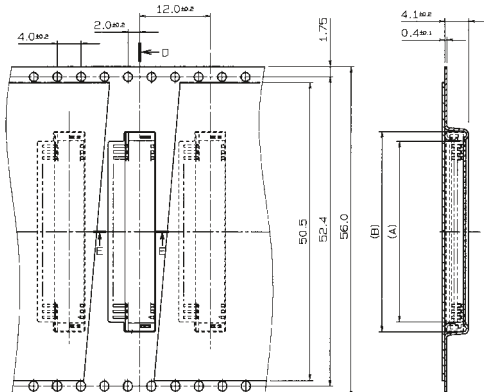
SECT. D-D
