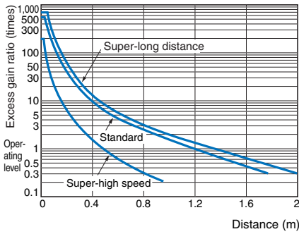
Operating Range Reflective E32-DC200
