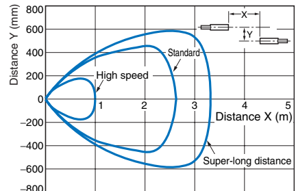
Through-beam E32-T11R
