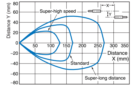
Through-beam E32-T14LR
