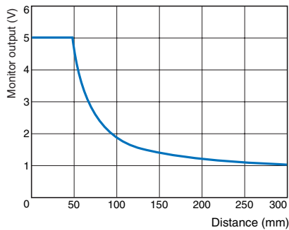
Through-beam E32-TC200
