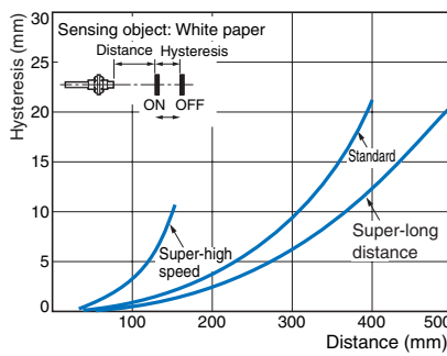
Hysteresis vs. Sensing Distance Reflective E32-D11L
