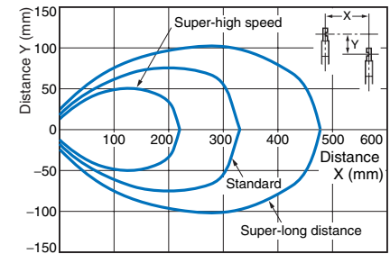
Through-beam E32-T14LR
