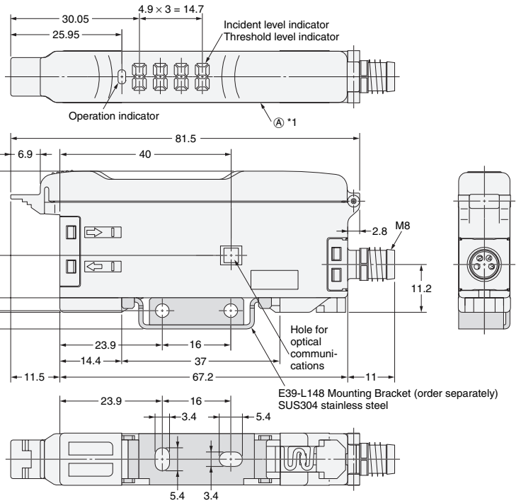
With Mounting Bracket Attached
