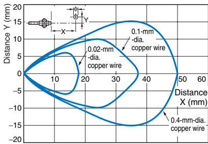
Operating Range Reflective E32-DC200
