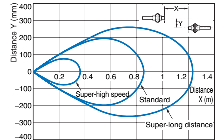
Through-beam E32-T22R
