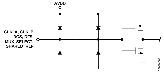
Figure 31. Equivalent Digital Input Circuit
