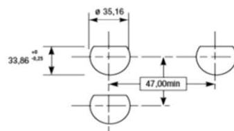
Panel Drilling
