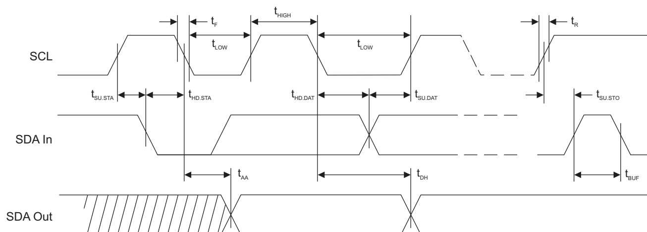
Figure 6-5. Bus Timing
