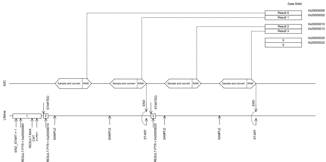
Figure 100: ADC
