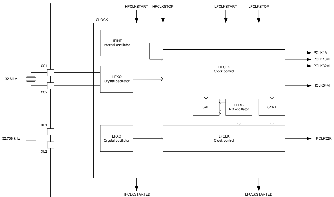
Figure 16: Clock control
