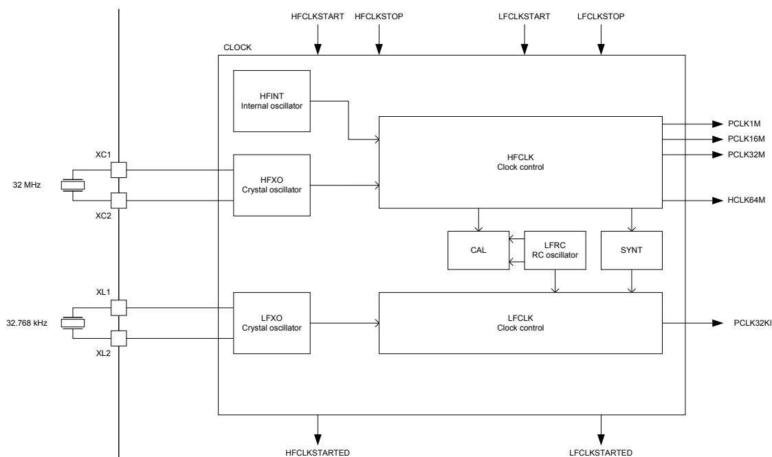
Figure 16: Clock control
