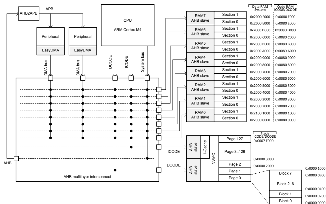
Figure 3: Memory layout
