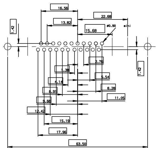
LAYOUT DIMENSIONS (after plating) CONNECTOR SIDE VIEW
