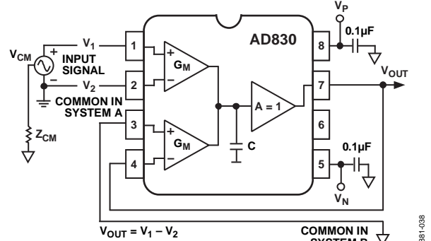
Figure 38. Differential Line Receiver
