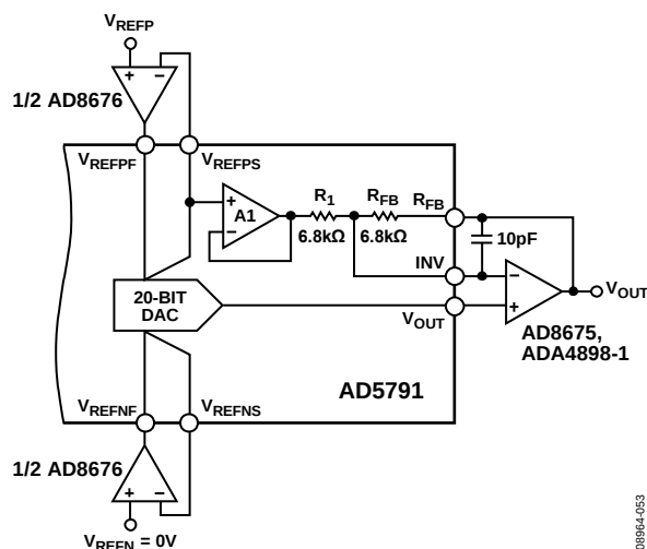
Figure 53. Output Amplifier in Gain of Two Configuration
