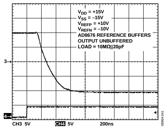
Figure 40. Falling Full-Scale Voltage Step
