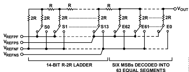
Figure 49. DAC Ladder Structure
