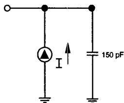
Figure 28. Test Load Configuration
