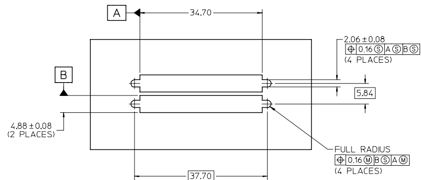
PANEL OPENING PER SFF-8441 SPECIFICATION SCALE 2:1
